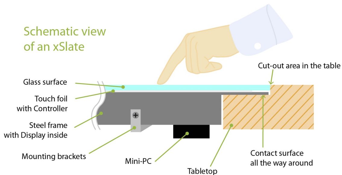
Fig. - Schematic structure of an xSlate table insert (not to scale)
